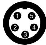
CAN BUS HARNESS
